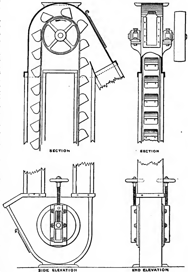
FIG. 14.—Grain Elevator.
