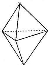
FIG. 75.—Trigonal Bipyramid.
