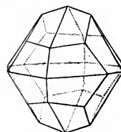
FIG. 35.—Dyakis-dodecahedron.
