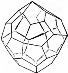
FIG. 40.—Pentagonal Icositetrahedron.
