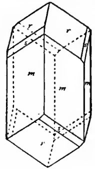
FIG. 76.—Crystal of Diopase.
