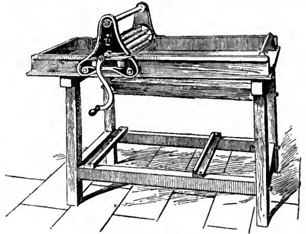
FIG. 16.—Butter-Worker.
