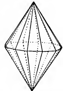
FIG. 77.—Dihexagonal Bipyramid.
