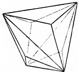
FIG. 28.—Triakis-tetrahedron.
