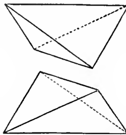
FIG. 50.—Tetragonal Bisphenoids.
