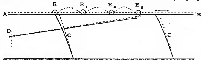
FIG. 8.—Swinging or Zimmer Conveyor.
