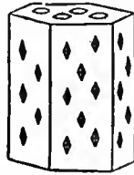
FIG. 92.—Nepheline. FIG. 93.—Calcite. FIG. 94.—Beryl. Etched Figures on Hexagonal Prisms.
